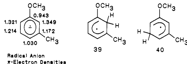
Figure 4. UHF/3-21G methoxytoluene radical anion densities and alternative protonated species.
