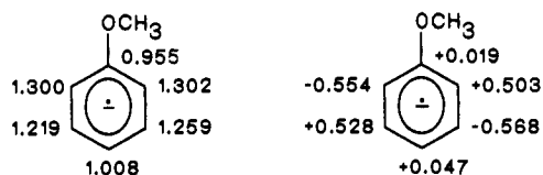
Radical Anion \pi -Electron Densities
