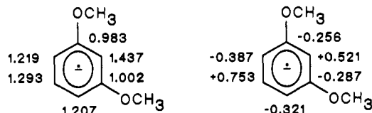
Radical Anion \pi -Electron Densities
